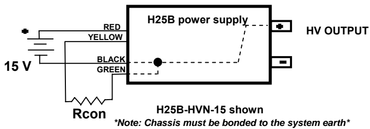
Figure 3: Resistance program of negative output of H25B
