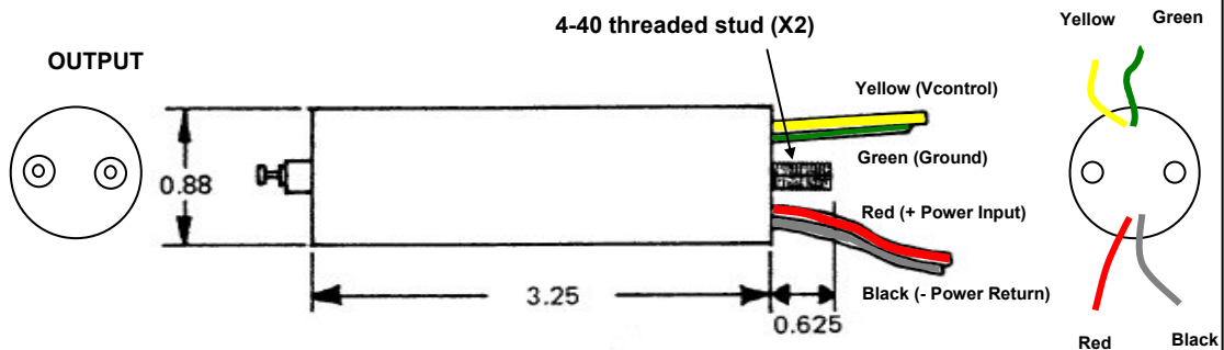
Cylindrical Configuration (H25B)
