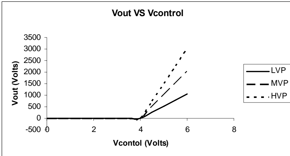
Figure 8: Negative Style H25B Output Voltage as a function of program voltage
