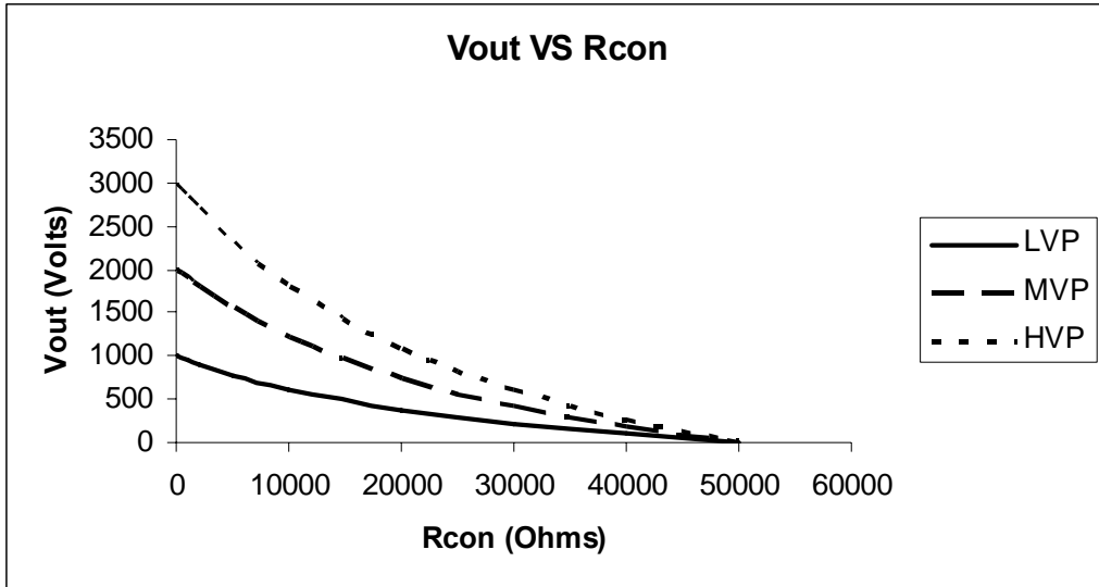
Figure 2: Positive Style H25B Output Voltage as a function of control resistor
