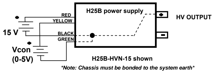
Figure 7: Voltage program of negative output of H25B
