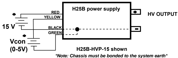
Figure 5: Voltage program of positive output of H25B
