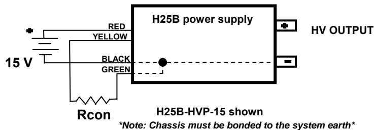
Figure 1: Resistance program of positive output of H25B
